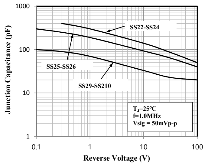
Fig.6 Typical Capacitance
