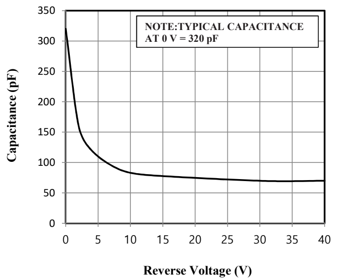
Fig.6 Typical Capacitance
